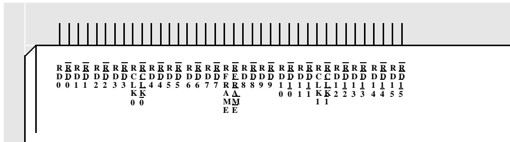
Figure 7-3. Recommended device pin escape, input port, top view of device
