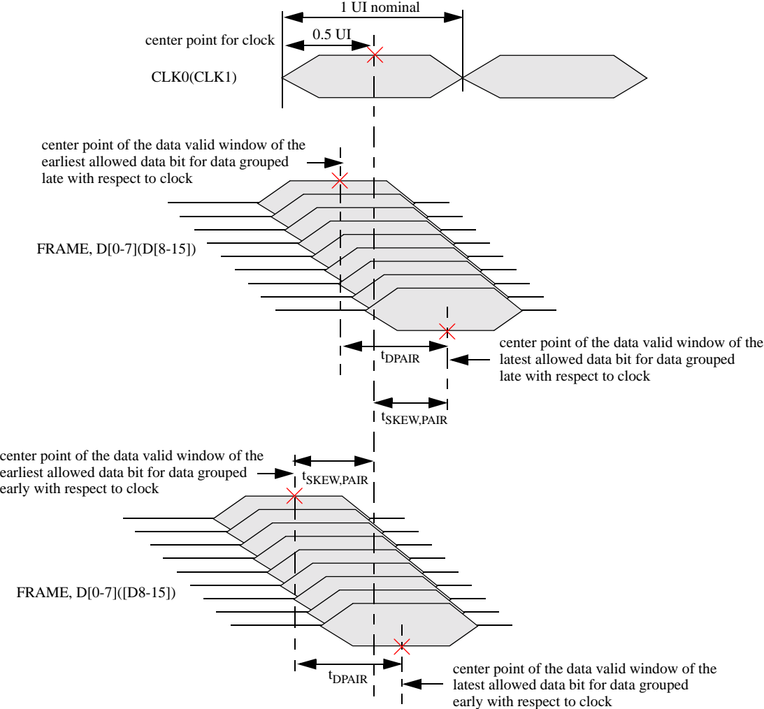
Figure 9-10. Static Skew Diagram
