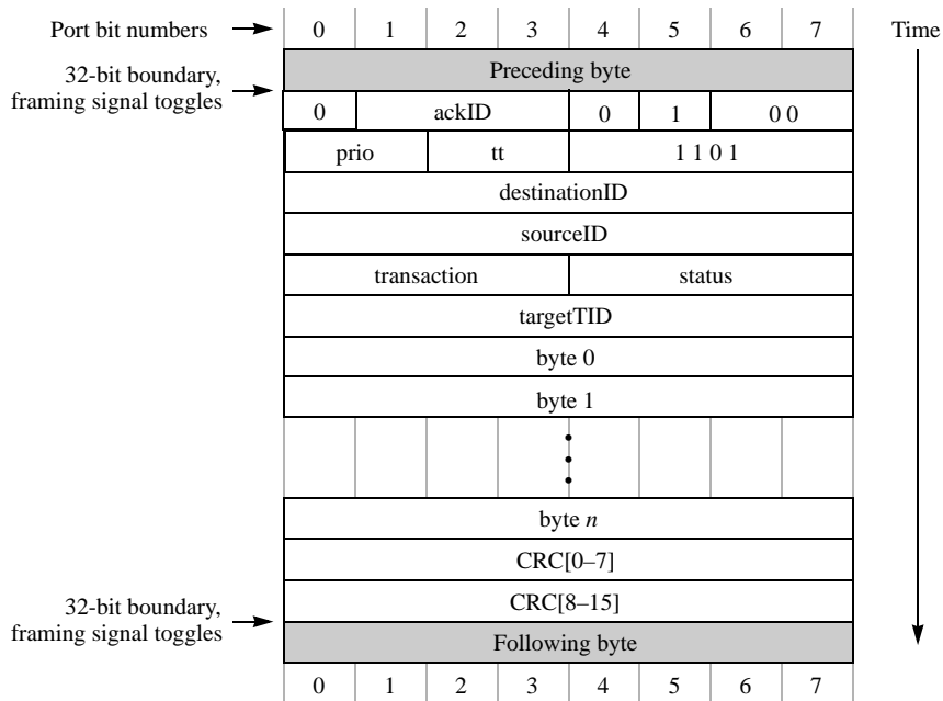
Figure 3-14. Response Packet Transmission Example 1
