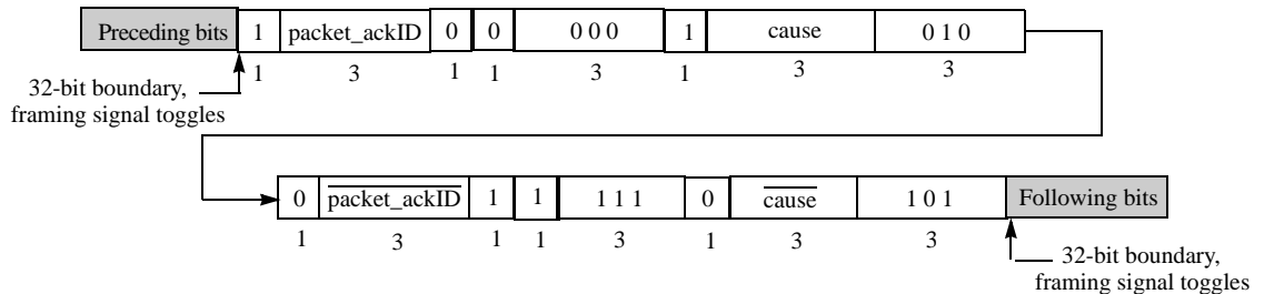
Figure 4-3. Type 2 Packet-Not-Accepted Control Symbol Format
