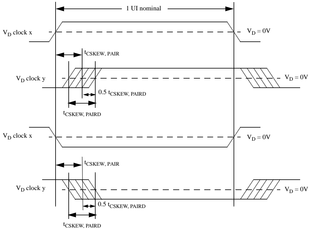
Figure 9-9. Clock to Clock Skew
