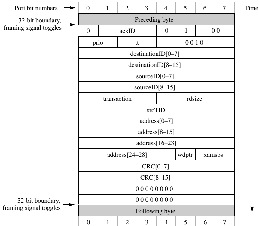
Figure 3-12. Request Packet Transmission Example 3
