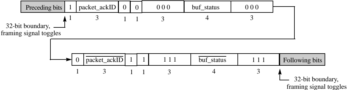
Figure 4-1. Type 0 Packet-Accepted Control Symbol Format
