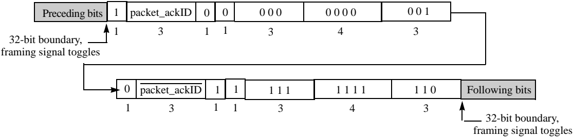
Figure 4-2. Type 1 Packet-Retry Control Symbol Format
