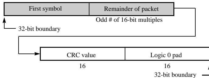
Figure 2-11. Padded Aligned Packet Bit Stream Example 1
