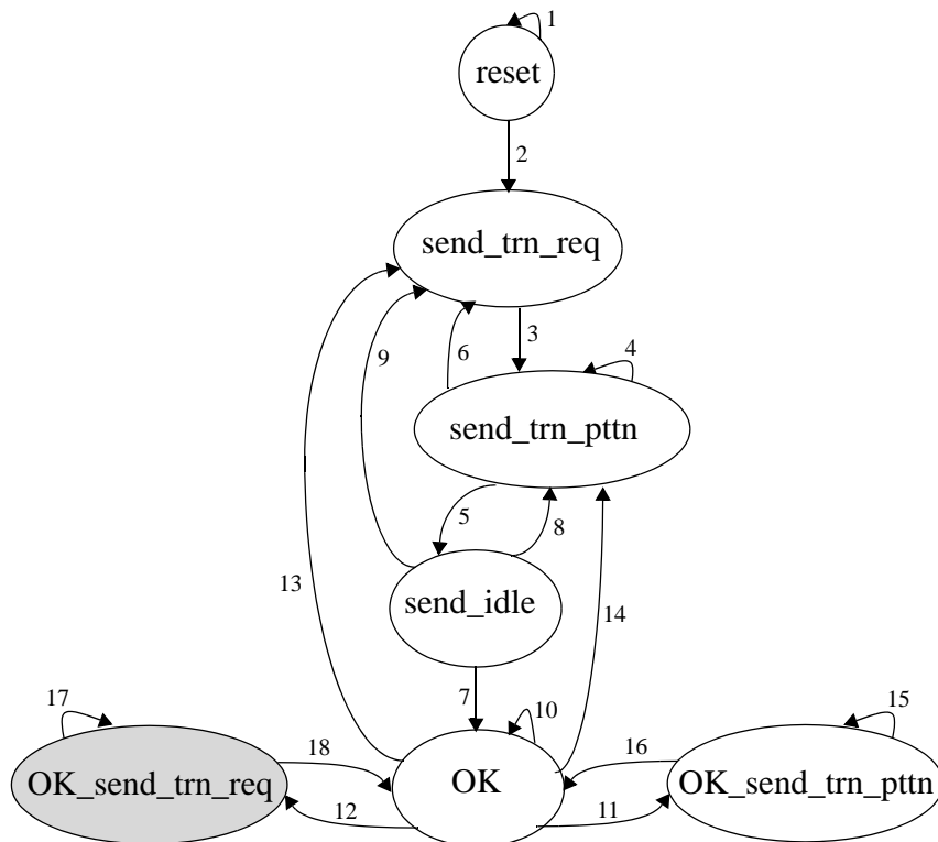
Figure A-2. Output port training state machine
