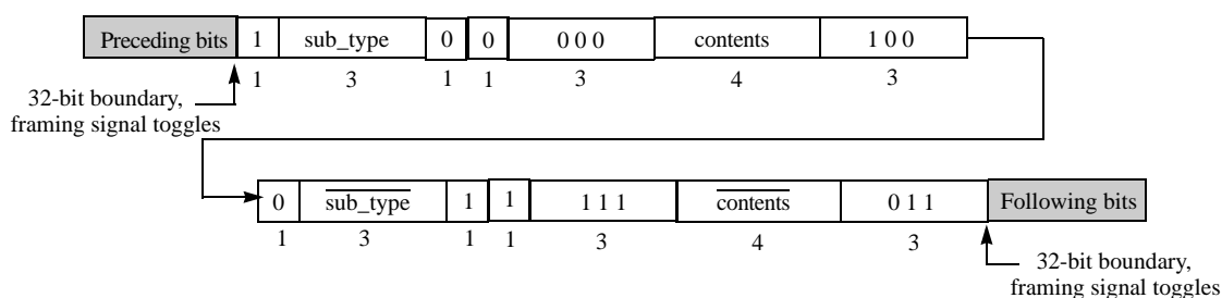
Figure 4-4. Type 4 Packet Control Symbol Format
